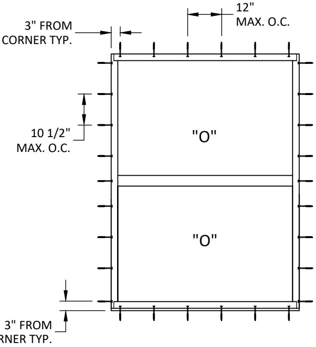
ANCHOR LAYOUT ALL INSTALLATIONS
