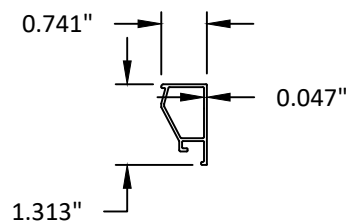
14 FIXED GLASS STOP
