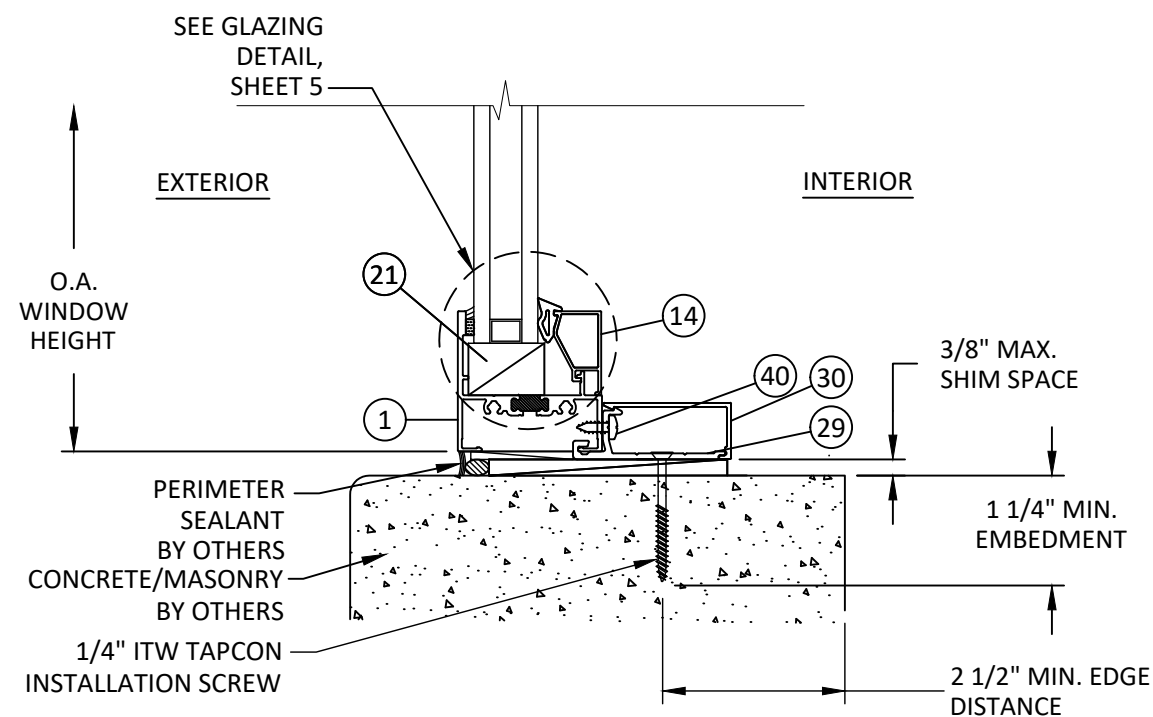
D 6 VERTICAL SECTION FIXED SILL - CONCRETE/MASONRY CLIP ANCHOR - TYP.
