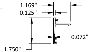
11 RECEPTOR STOP
