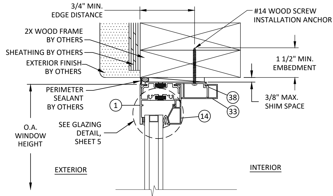
H7 VERTICAL SECTION FIXED HEAD - 2X WOOD FRAME STRAP ANCHOR - TYP.
