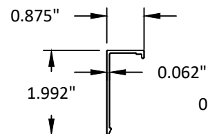
30 ANCHOR CLIP
