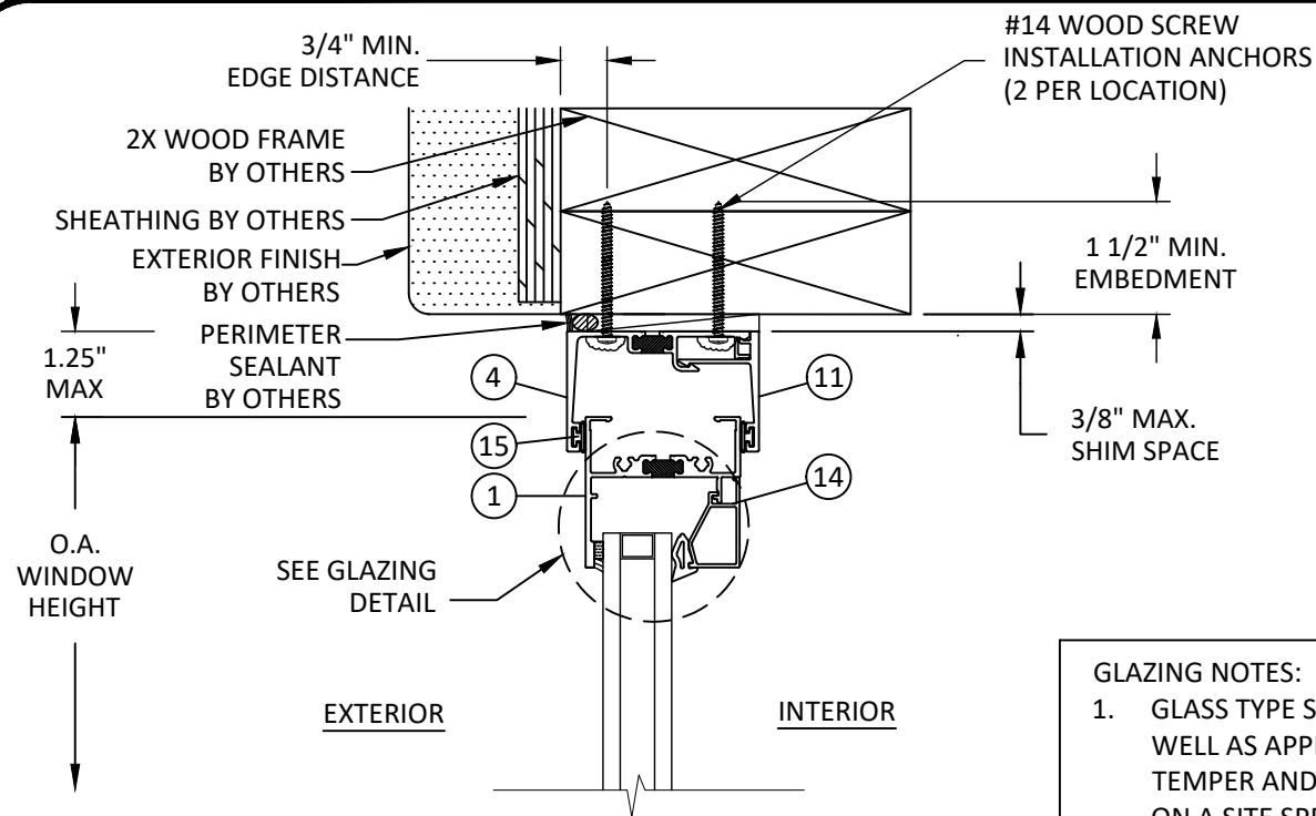
B 5 VERTICAL SECTION FIXED HEAD - 2X WOOD FRAME INT. SET RECEPTOR - TYP.
