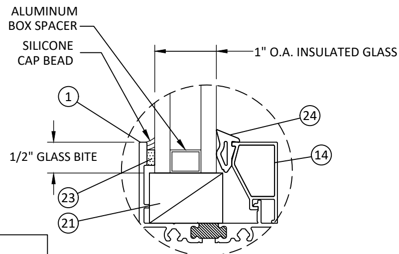
FIXED GLAZING DETAIL
