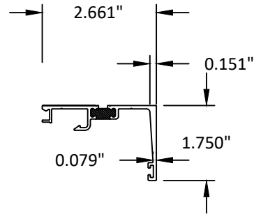
4 RECEPTOR
