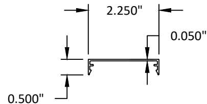
12 COVER
