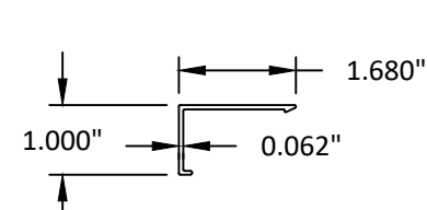
35 1" X 1 11/16" COVER
