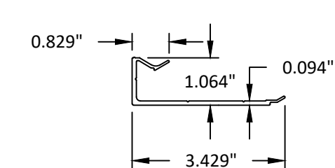
36 1 1/8" X 3 1/2" CLIP
