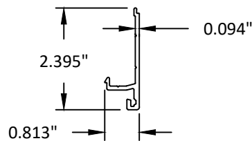
29 ANCHOR CLIP
