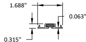
26 THROUGH FRAME FILLER PLATE
