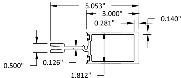
10 STACKING MULLION
