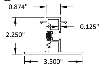
48 INTEGRAL MULL
