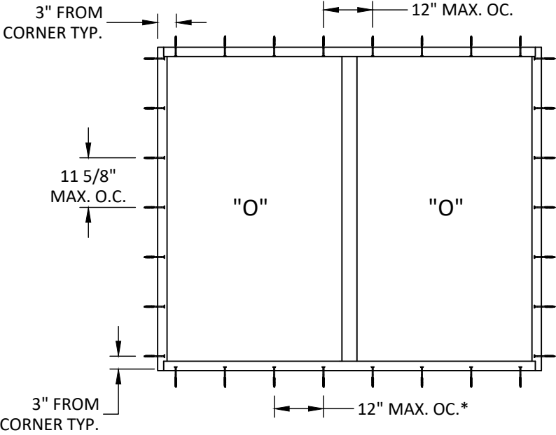
ANCHOR LAYOUT ALL INSTALLATIONS
