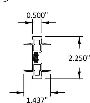
51 I MULLION
