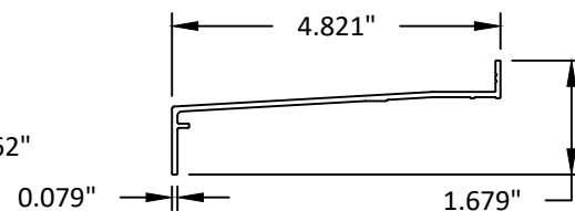
54 4" SILL TRIM
