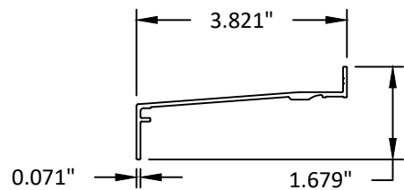
8 3" SILL TRIM
