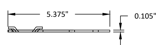
50 TWIST ANCHOR
